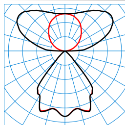
Creavo H3-L LW19-03 89-840 ETDD X4 01 TX278431
