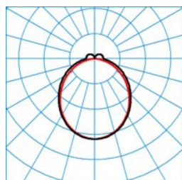
ELINE DSL35-100 ML 840 L150 4 50
