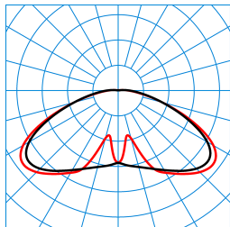
Publisca P1W-RBT/1800-730 2G1S ETDD (CLO initial value) TX301122
