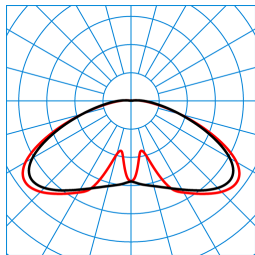
Publisca P1W-RBT/1800-730 2G1S ETDD (CLO end value) TX300344
