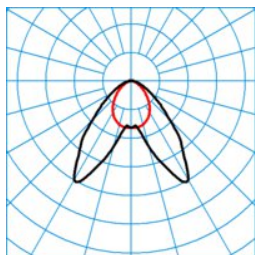
ELINE HE LDAH40-120 ML 840 L150 2 50 ■ C0 - C180
