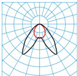
ELINE HE LDAH40-120 ML 840 L150 4 50 ■ C0 - C180
