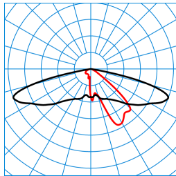
Publisca P1W-AB2L/2200-730 3G1S TX053465
