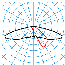
Publisca P1W-AB2L/2200-730 3G1S ETDD (CLO initial value) TX300870
