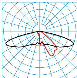
Publisca P1W-AB2L/2200-730 3G1S ETDD (CLO end value) TX301024
