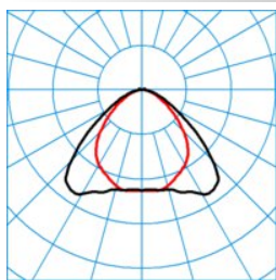
ELINE HE LVW60-160 ML 830 L225 0 50 ■ C0 - C180
