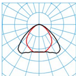
ELINE HE LVW60-160 ML 830 L225 2 50 ■ C0 - C180
