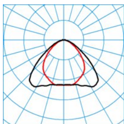
ELINE HE LVW60-160 ML 830 L225 4 50 ■ C0 - C180
