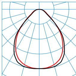
ArimoFit M73 PW19 42-8TW ETDD8 TWW + ArimoFit Sky M73-TS ZER (DWW) TX874703
