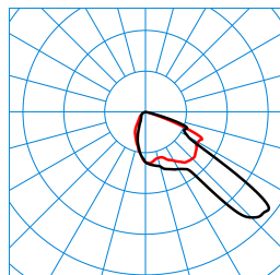
LIQ 50N-FR1L/5600-722 6G1 ET (CLO end value) TX780622
