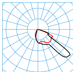
LIQ 50N-FR1L/5600-722 6G1 ET (CLO initial value) TX780628
