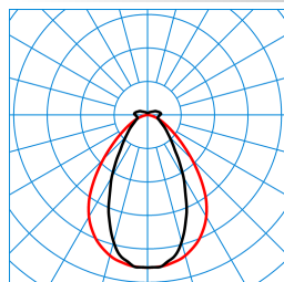
TugraHE+ 12 PN 80-940 ETDD PC 23 TX558382
