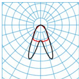
ELINE HE LDAN60-160 ML 865 L225 2 20 ■ C0 - C180
