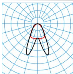
ELINE HE LDAN60-160 ML 865 L225 0 20 ■ C0 - C180
