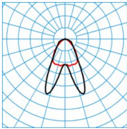
ELINE HE LDAN60-160 ML 865 L225 2 20
