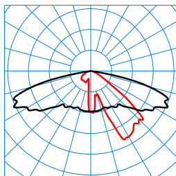
Publisca P1W-AB2L/1800-740 2G1S ETDD (CLO initial value) TX300492
