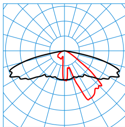
Publisca P1W-AB2L/1800-740 2G1S ETDD (CLO end value) TX301018
