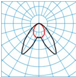
ELINE HE LDAH40-120 ML 830 L150 4 20 ■ C0 - C180
