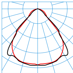
SFlow C2-L MRW LED4000-830 ET 01 TX771493
