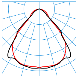
SFlow C2-L MRW LED4000-830 ET 01 TX721384
