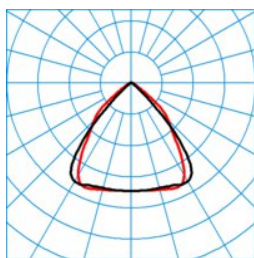
ELINE HE LW2240-120 ML 840 L150 2 20 ■ C0 - C180
