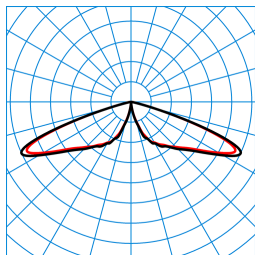
CS 19 100-RB6L-SLR1/5100-730 4G1S ET (CLO initial value) TX299935
