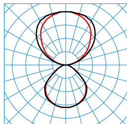
Luceos D/H2-L CDP 6500-830 ETDD 01 (Pendant ZS/ZST) TX877255
