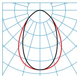
ArmoFit M73 DW19 42-8TW ETDD8 + ArmoFit Sky M73-TS ZER (DWW) TX874826
