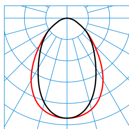
ArmoFit M73 DW19 42-8TW ETDD8 (DCW) TX874834
