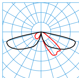
CS 19 100-AB2L/3200-740 4G1S ETDD (CLO initial value) TX300017
