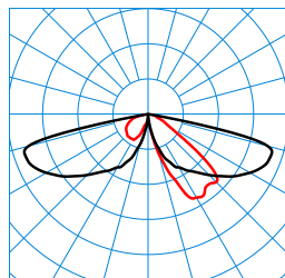
CS 19 100-AB2L/3200-740 4G1S ETDD (CLO end value) TX300016
