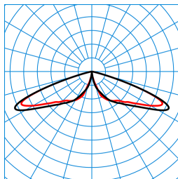
CS 19 100-RB6L/2200-740 2G1S ETDD (CLO initial value) TX300062
