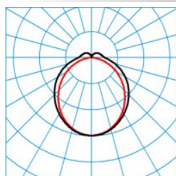
ELINE HE DL80 827 L225 2 20
