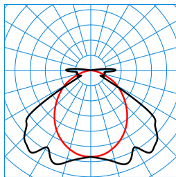
Nextrema G3 B 60-840 ETDD +HFSB TWP TX768603
