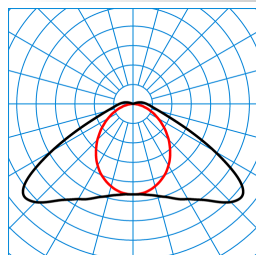
Nextrema G3 XB 6000-840 ET +HFS PC TX770673
