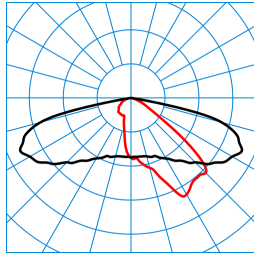
LIQ 50N-AB2L-LRA/1200-722 2G1 ETDD (CLO end value) TX776415
