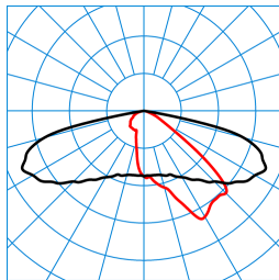
LIQ 50N-AB2L-LRA/1200-722 2G1 ETDD (CLO initial value) TX776416
