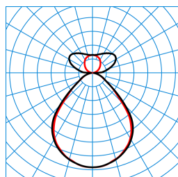
Opendo H1-L PW19 20-53/6/ML-830 ET 03 (2100lm) TX376526
