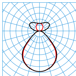
Opendo H1-L PW19 20-53/6/ML-830 ET 03 (3200lm) TX376528
