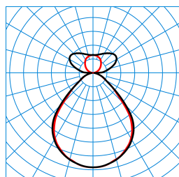
Opendo H1-L PW19 20-53/6/ML-830 ET 03 (2900lm) TX376527
