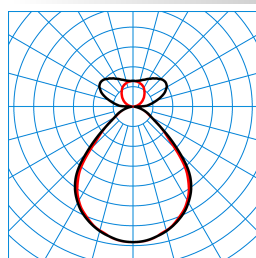
Opendo H1-L PW19 20-53/6/ML-830 ET 03 (1900lm) TX376525
