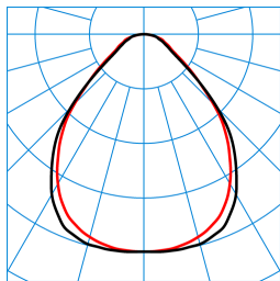
ArimoFit G2 D PW19-X 42-840 ETDD 03/03 TX377156
