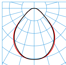
Belviso C1 M46 CDP LED3800ww ETDD TX773373
