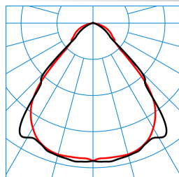
SFlow D1-L MRW LED3200-840 ET 03 TX769627
