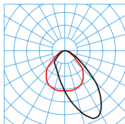
Luceos D/H2-L CDP-A 5000-830 ETDD 03 (Pendant ZS/ZST) TX877268
