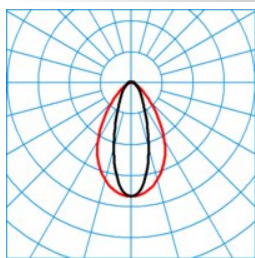
ELINE HE PN55-150 ML 830 L225 0 20
