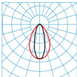
ELINE HE PN55-150 ML 830 L225 4 20
