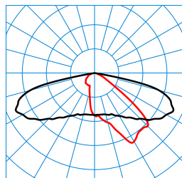
LIQ 50N-AB2L-LR/5600-730 6G1 ET (CLO end value) TX777999
