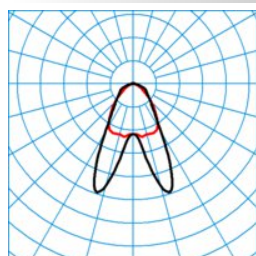
ELINE HE LDAN80 827 L150 2 20 ■ C0 - C180 DIN 5040 = A50 UGR I = 23,1 UGR q = 23,8 UTE = 0.99 C + 0.01 T CEN flux code = 64 88 97 99 100 0 7 47 1
