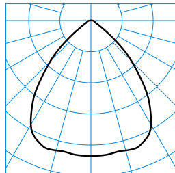
InperiaL G2 C07 BR22 1800-840 03 + ZN-PC TX052892
