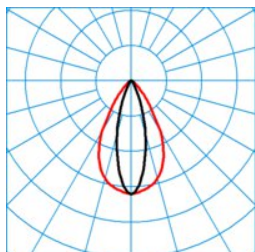
ELINE LEN55-140 ML 830 L225 4 50
