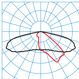
LIQ 50N-AB2L-LR-SLR2/2200-730 2G1 ET (CLO initial value) TX777081
