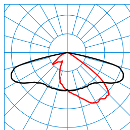
LIQ 70N-AB7L-LRA/10/12/135-730 12G1 ETDD (CLO initial value) TX27885
