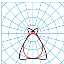
ELINE HE PMW2230-100 ML 865 L150 0 20 ■ C0 - C180
