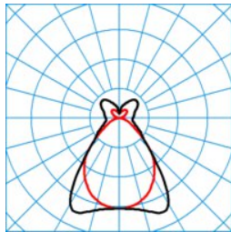
ELINE HE PMW2230-100 ML 865 L150 4 20 ■ CO - C180 DIN 5040 = B52 UGR I 3 = 17,3 UGR q 3 = 20,4 UTE 3 = 0.72 D + 0.28 T CEN flux code = 60 83 94 72 100 26 58 82 28
