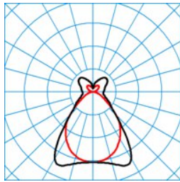
ELINE HE PMW2230-100 ML 865 L150 2 20 ■ CO - C180 DIN 5040 = B52 UGR I 3 = 16,6 UGR q 3 = 19,7 UTE 3 = 0.72 D + 0.28 T CEN flux code = 60 83 94 72 100 26 58 82 28
