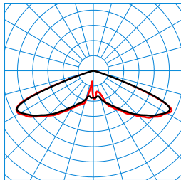
Publisca P1W-RB6L-LRA/2600-730 3G1S ET (CLO initial value) TX300751
