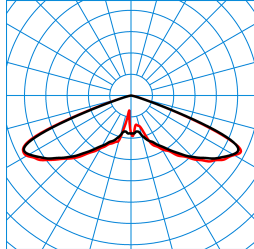
Publisca P1W-RB6L-LRA/2600-730 3G1S TX053547
