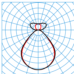
Opendo H2-L PW19 57-8TW ETDD8 03 (DWW) TX874581
