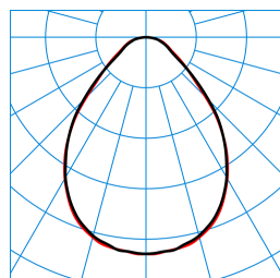
ArimoFit M48 PW19 53-8TW ETDD8 + ArimoFit Sky M48-TS ZER (DWW) TX874658
