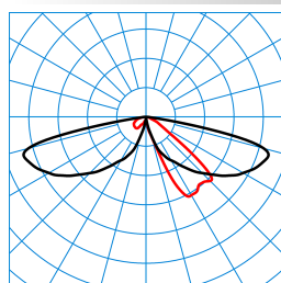
LTX Z-AB2L-LRA/15/18/26-740 4G1 (1800 lm) TX062709
