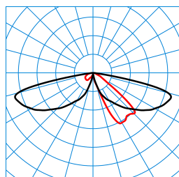
LTX Z-AB2L-LRA/15/18/26-740 4G1 (1500 lm) TX059701
