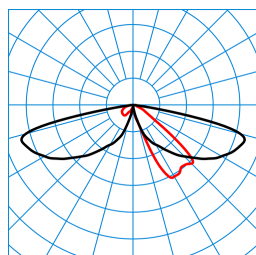
LTX Z-AB2L-LRA/15/18/26-740 4G1 (2600 lm) TX062710
