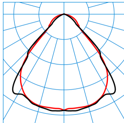
SFlow D2-L MRW LED4000-8TW ETDD8 01 (DCW) TX877102
