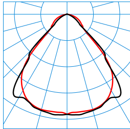
SFlow D2-L MRW LED4000-8TW ETDD8 01 (DWW) TX877077
