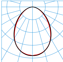
SFlow C2-L MRWD LED4000-830 ETDD 01 TX771513
