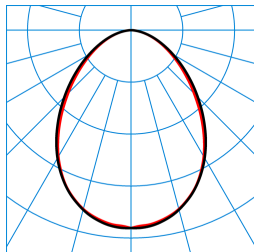
SFlow C2-L MRWD LED4000-830 ETDD 01 TX721368
