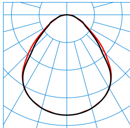
Siella G8 M84 PW19 28-44/4ML-840 ETDD (stage 2) TX562702
