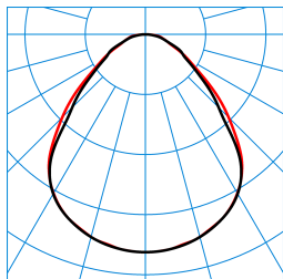
Siella G8 M84 PW19 28-44/4ML-840 ETDD (stage 3) TX562633
