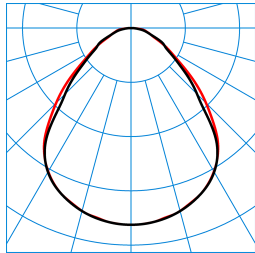
Siella G8 M84 PW19 28-44/4ML-840 ETDD (stage 1) TX562642
