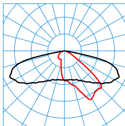
LIQ 50N-AB2L-LR/350/420/460-727 6G1 ET (CLO initial value) TX777751
