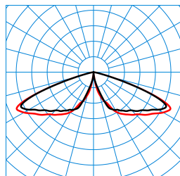
CS 19 C 100-RB6L/1800-730 2G1S ETDD (CLO end value) TX299924
