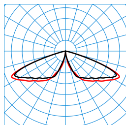
CS 19 C 100-RB6L/1800-730 2G1S ETDD (CLO initial value) TX299925
