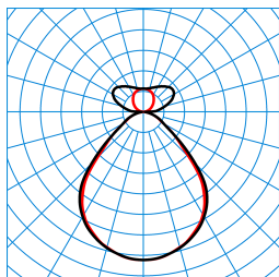
Opendo H2-L PW19 20-64/6/ML-830 ET 03 (3400lm) TX376591
