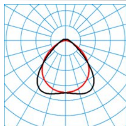
ELINE HE PW180 865 L225 1 20
