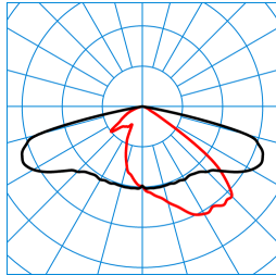
LIQ 70N-AB7L-LRA/10000-722 12G1 ETDD (CLO end value) TX778446
