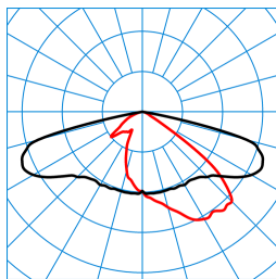
LIQ 70N-AB7L-LRA/10000-722 12G1 ETDD (CLO initial value) TX778454
