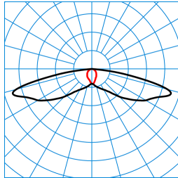
LIQ 50N-SB3L-LRA/1000-722 2G1 ETDD (CLO end value) TX775925
