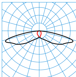
LIQ 50N-SB3L-LRA/1000-722 2G1 ETDD (CLO initial value) TX775926
