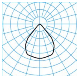
SNS RC5-MR1XFL-20-830
